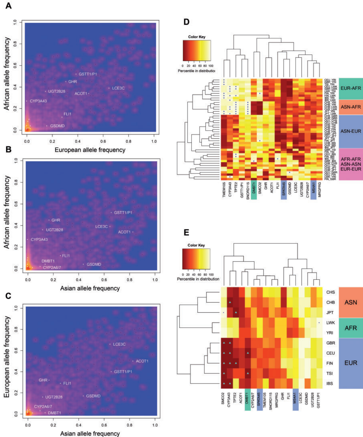
FIG. 4. Analysis of exonic variants. (A–C) The allele frequency of exonic deletion variants. The x - and y axes indicate the allele frequencies in a given continent. The heatmap colors represent number of observations. The red to dark blue gradient corresponds to decreased density of observed deletions. Here, we plot allele frequencies of all 14,422 1KG deletion variants. As such, red spots designate thousands of observations decreasing to hundreds of observations for yellow pixels and single observations for purple dots. A vast majority of deletions have very low allele frequencies. The exonic variants shared with Neanderthal/Denisovan genomes are shown with white-colored circles. (D) Heatmap of the percentiles of pairwise F_{ST} values measured for the flanking regions of the ancient exonic deletion variants between ten nonadmixed populations using clustering without a priori input. The colors in the heatmap correspond to the percentile of the F_{ST} values as compared with the distribution of all exonic human deletions, with light-yellow/white being the highest values observed (1 indicating the highest percentile) and dark red corresponding to lower values (0 indicating the lowest possible percentile). Exact values to generate this map can be found in supplementary table S2, Supplementary Material online. On the x axis are the exonic deletion variants, represented by the names of the genes that they affect. The ones highlighted in blue are introgressed deletions, the one highlighted in green is a recurrent deletion, and those that are not highlighted are ancient deletions. On y axis are population pairs used in the analysis. AFR, African; ASN, Asian; EUR, European; CEU, Utah residents (CEPH) with Northern and Western European ancestry; CHB, Han Chinese in Beijing; CHS, Southern Han Chinese; FIN, Finish in Finland; GBR, British in England and Scotland; IBS, Iberian population in Spain; JPT, Japanese in Tokyo; LWK, Luhya in Webuye, Kenya; TSI, Toscani in Italia; YRI, Yoruba in Ibadan, Nigeria. (E) Heatmap of the percentiles of Tajima's D values observed for ancient exonic deletion variants within the Tajima's D distribution of all exonic human deletions. The colors in the heatmap correspond to the percentile
